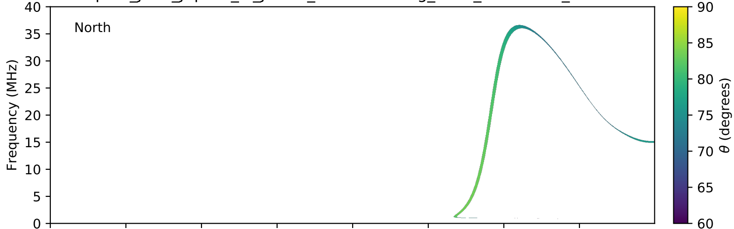
expres_juno_jupiter_io_jrm09_lossc-wid1deg_3kev_20161220_v01.cdf
