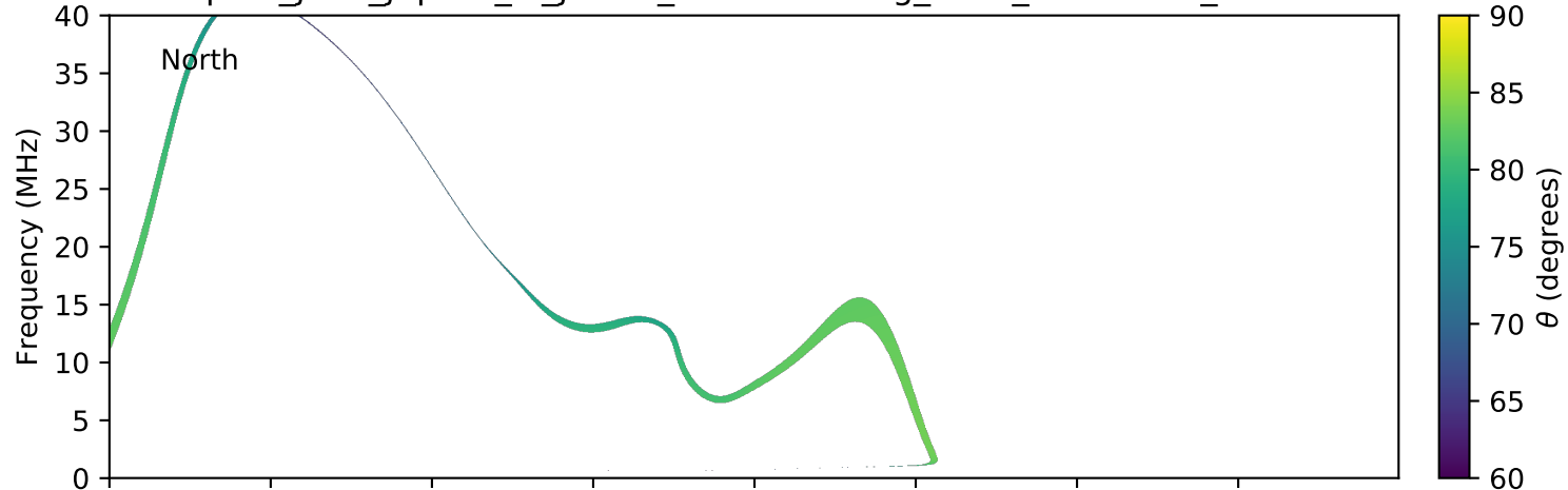
expres_juno_jupiter_io_jrm09_lossc-wid1deg_3kev_20161219_v01.cdf
