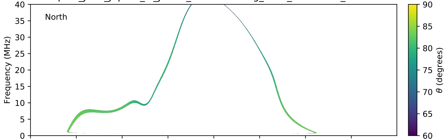
expres_juno_jupiter_io_jrm09_lossc-wid1deg_3kev_20161217_v01.cdf
