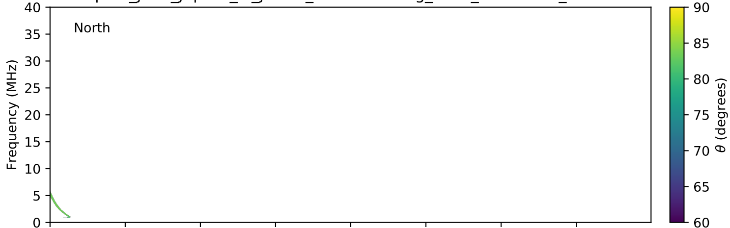
expres_juno_jupiter_io_jrm09_lossc-wid1deg_3kev_20161216_v01.cdf
