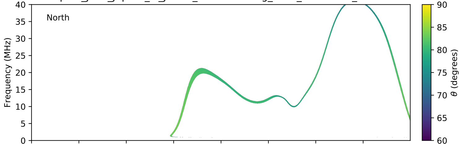
expres_juno_jupiter_io_jrm09_lossc-wid1deg_3kev_20161215_v01.cdf
