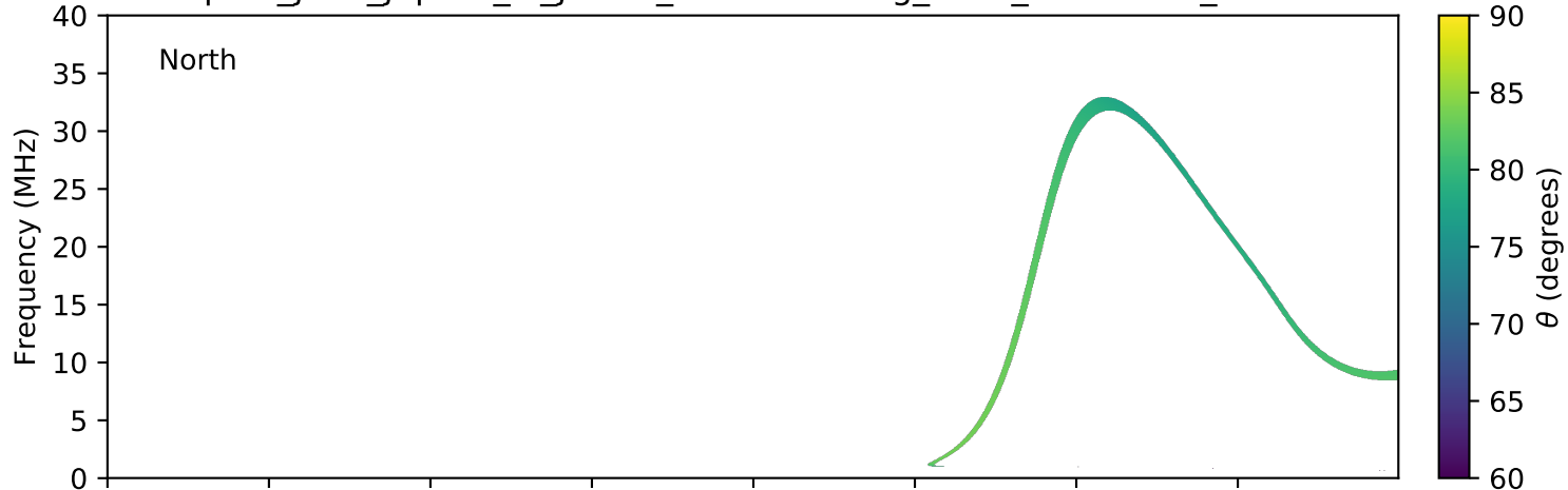
expres_juno_jupiter_io_jrm09_lossc-wid1deg_3kev_20161213_v01.cdf
