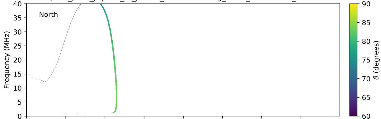
expres_juno_jupiter_io_jrm09_lossc-wid1deg_3kev_20161207_v01.cdf
