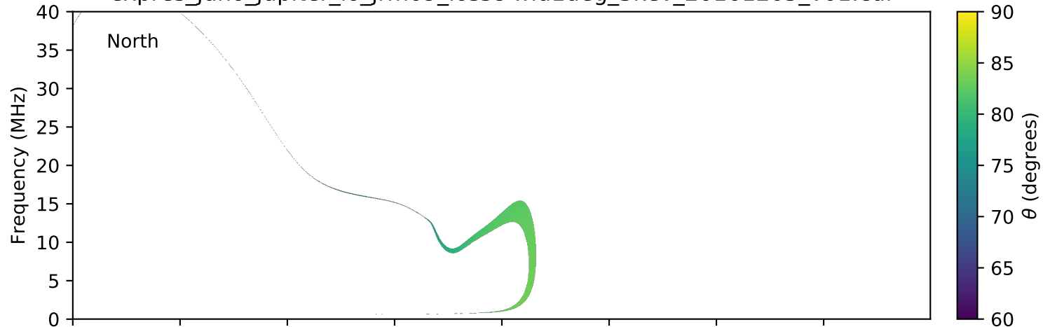
expres_juno_jupiter_io_jrm09_lossc-wid1deg_3kev_20161205_v01.cdf
