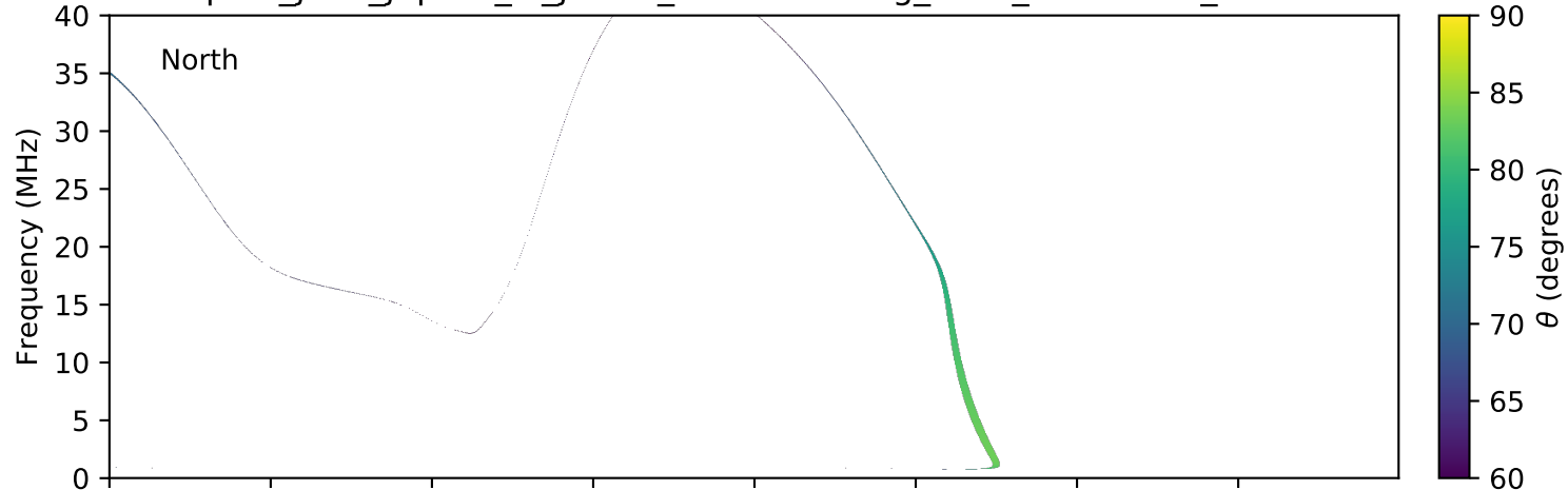
expres_juno_jupiter_io_jrm09_lossc-wid1deg_3kev_20161203_v01.cdf
