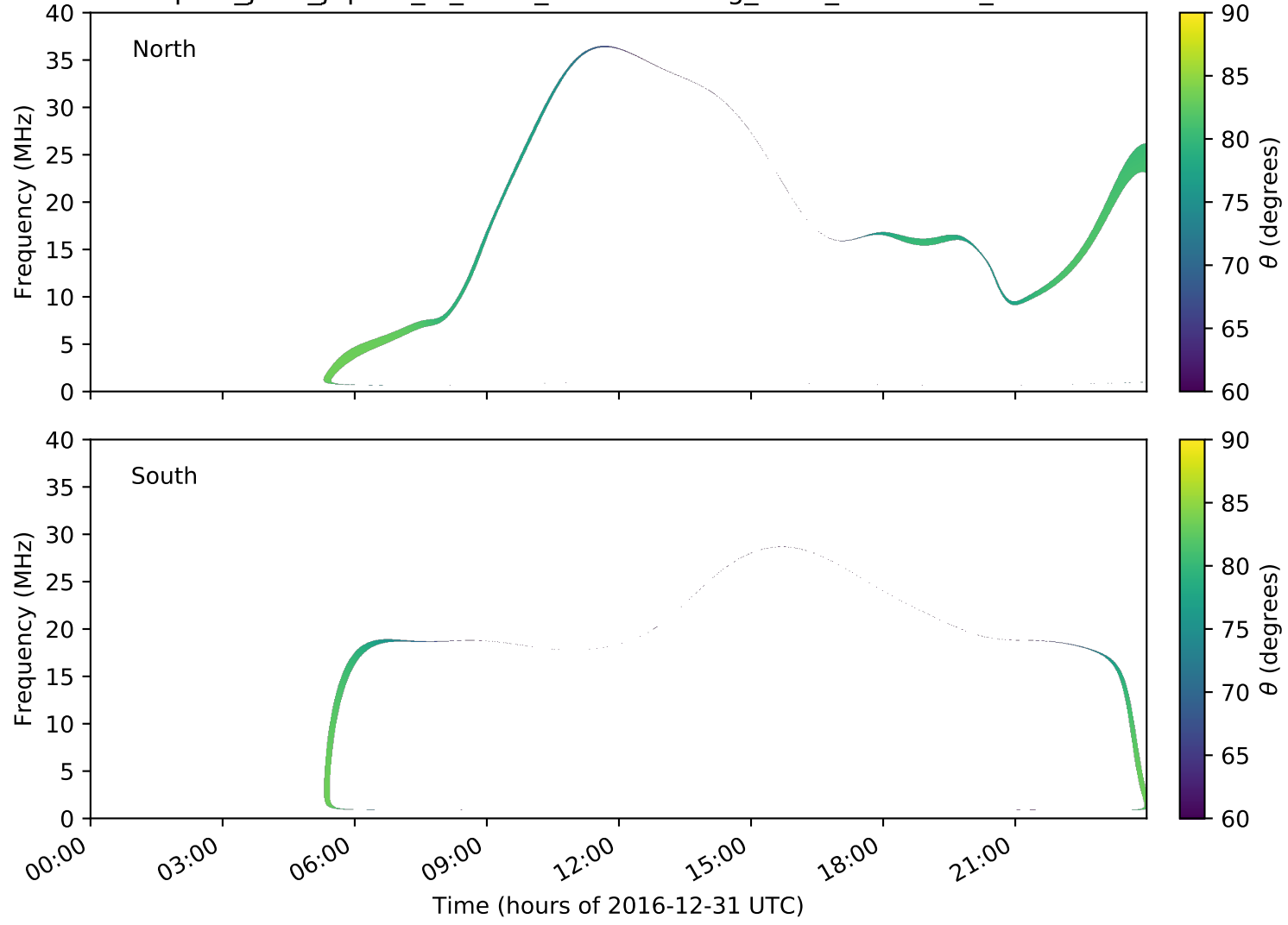
expres_juno_jupiter_io_isaac_lossc-wid1deg_3kev_20161231_v01.cdf
