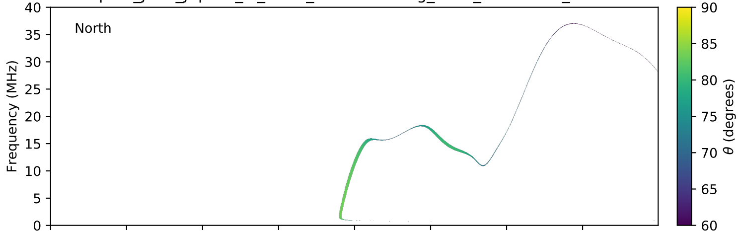
expres_juno_jupiter_io_isaac_lossc-wid1deg_3kev_20161229_v01.cdf
