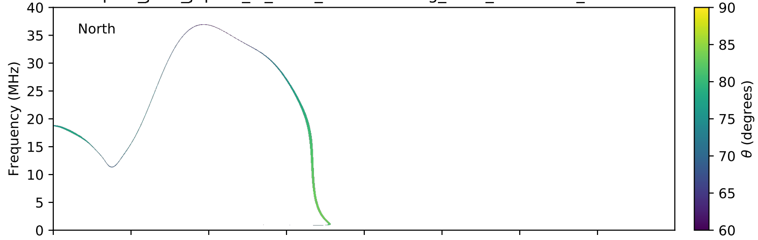
expres_juno_jupiter_io_isaac_lossc-wid1deg_3kev_20161228_v01.cdf
