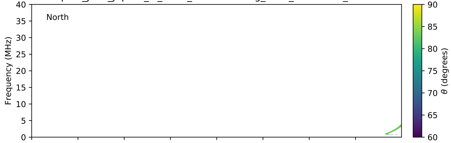
expres_juno_jupiter_io_isaac_lossc-wid1deg_3kev_20161225_v01.cdf
