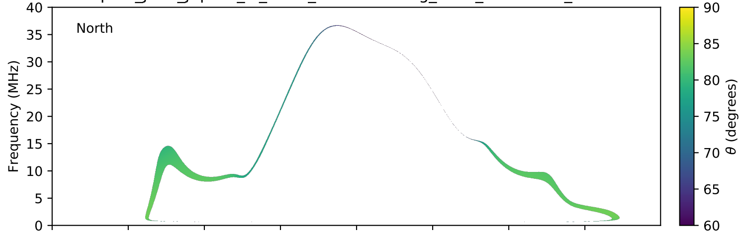
expres_juno_jupiter_io_isaac_lossc-wid1deg_3kev_20161224_v01.cdf
