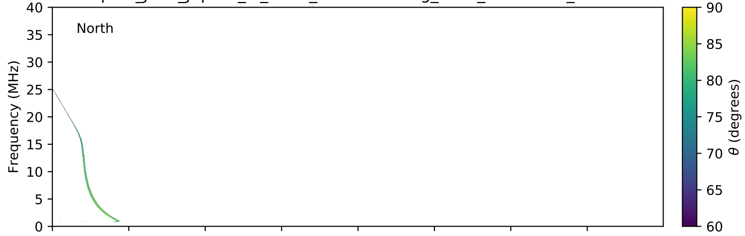
expres_juno_jupiter_io_isaac_lossc-wid1deg_3kev_20161223_v01.cdf
