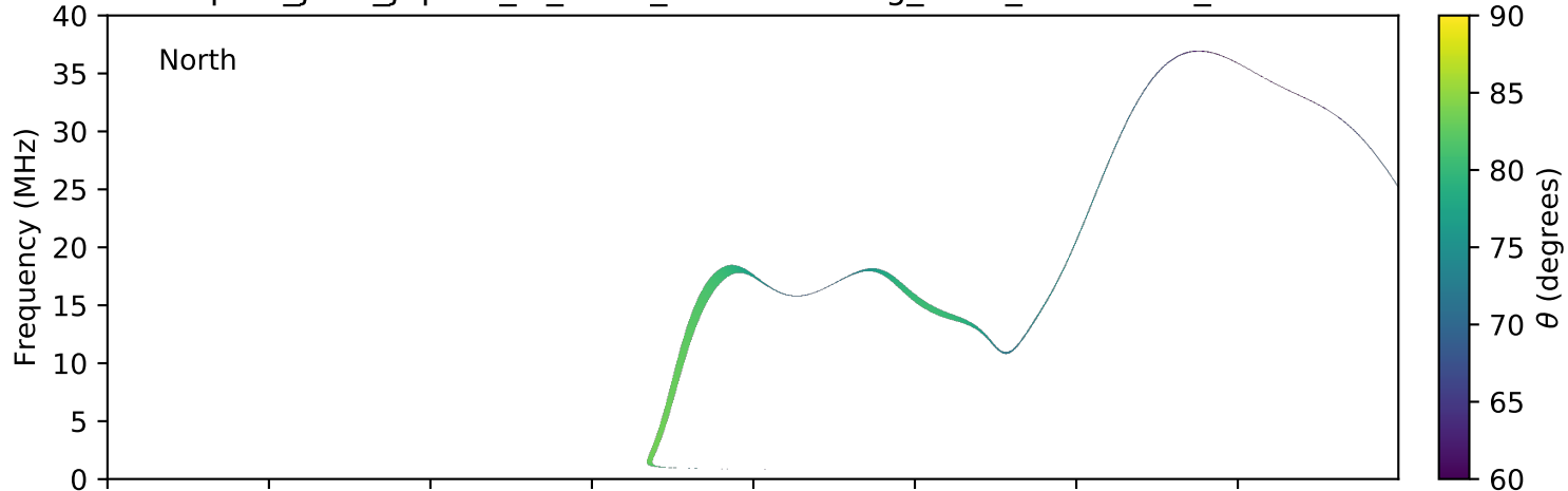
expres_juno_jupiter_io_isaac_lossc-wid1deg_3kev_20161222_v01.cdf
