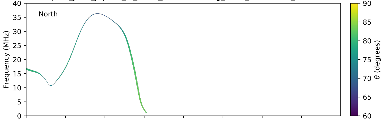
expres_juno_jupiter_io_isaac_lossc-wid1deg_3kev_20161221_v01.cdf
