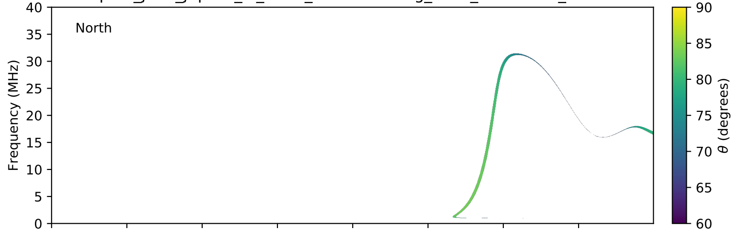
expres_juno_jupiter_io_isaac_lossc-wid1deg_3kev_20161220_v01.cdf
