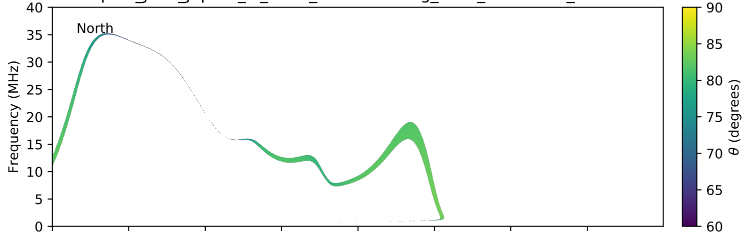
expres_juno_jupiter_io_isaac_lossc-wid1deg_3kev_20161219_v01.cdf
