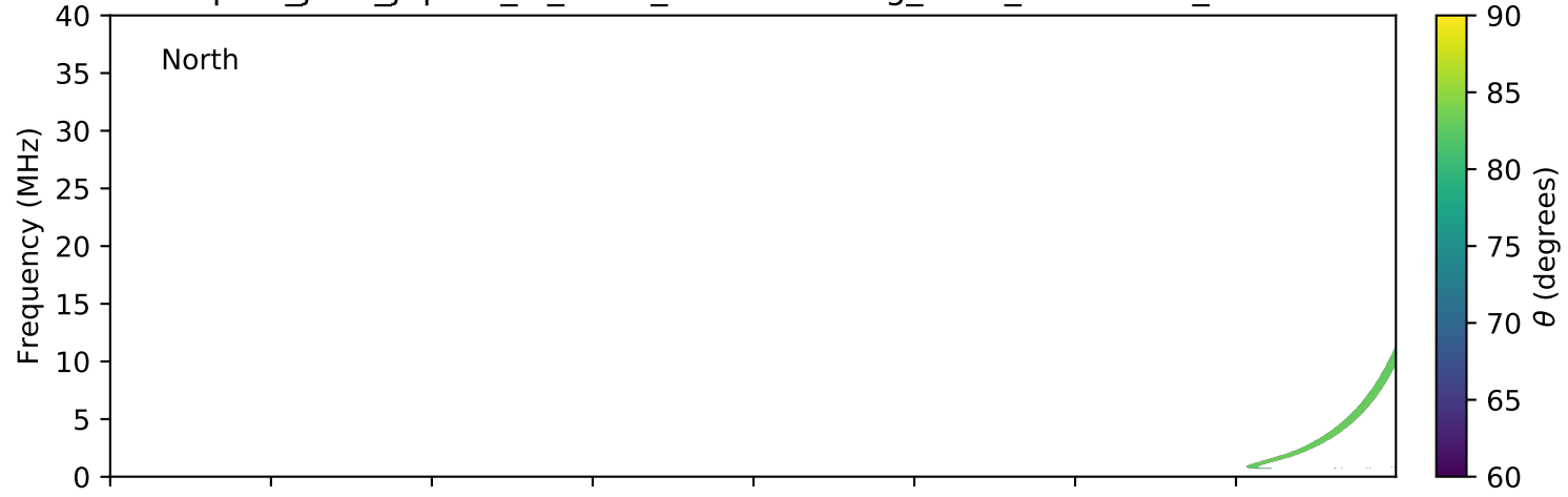
expres_juno_jupiter_io_isaac_lossc-wid1deg_3kev_20161218_v01.cdf
