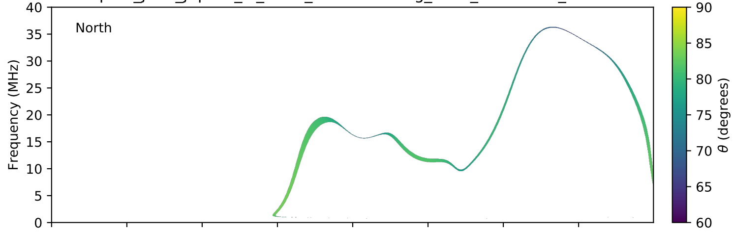
expres_juno_jupiter_io_isaac_lossc-wid1deg_3kev_20161215_v01.cdf
