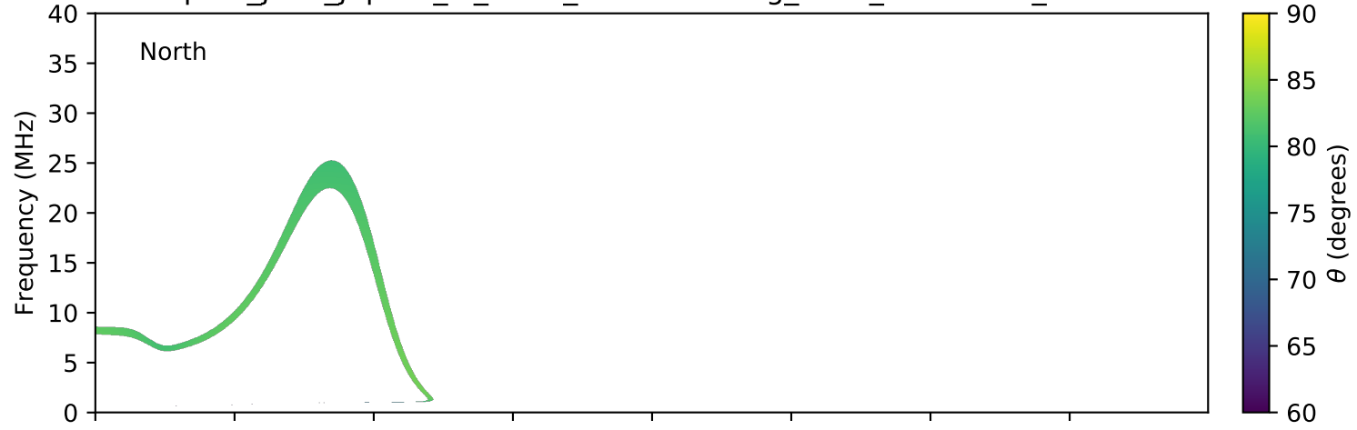
expres_juno_jupiter_io_isaac_lossc-wid1deg_3kev_20161214_v01.cdf
