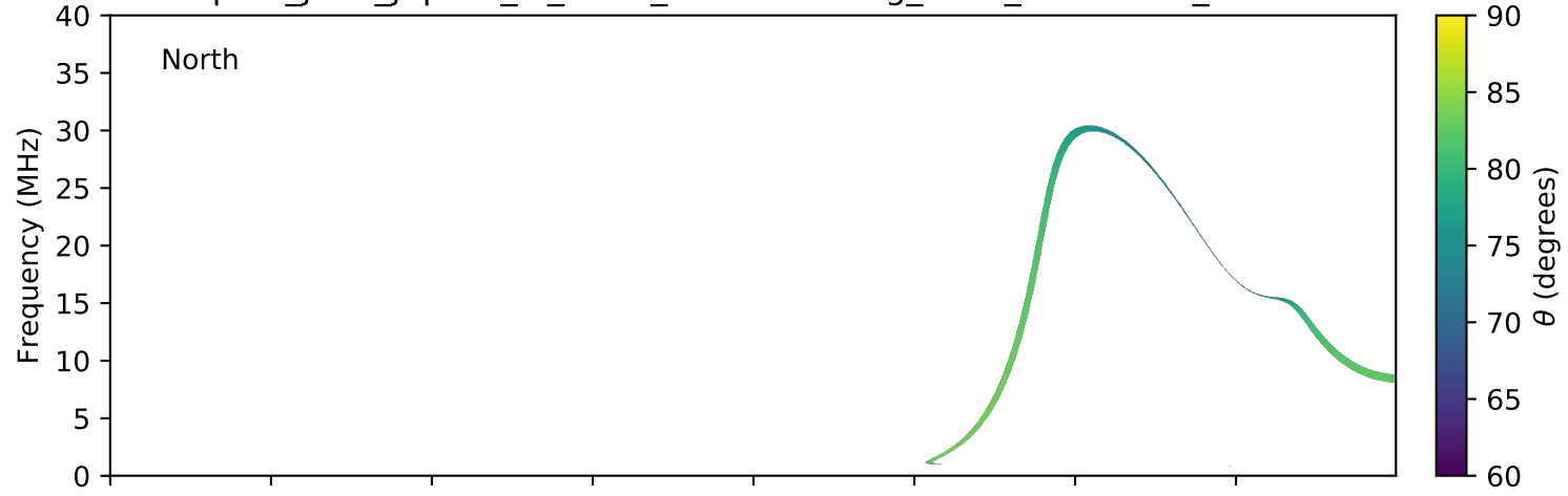
expres_juno_jupiter_io_isaac_lossc-wid1deg_3kev_20161213_v01.cdf
