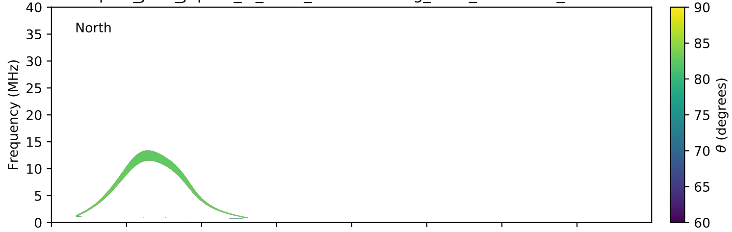
expres_juno_jupiter_io_isaac_lossc-wid1deg_3kev_20161212_v01.cdf
