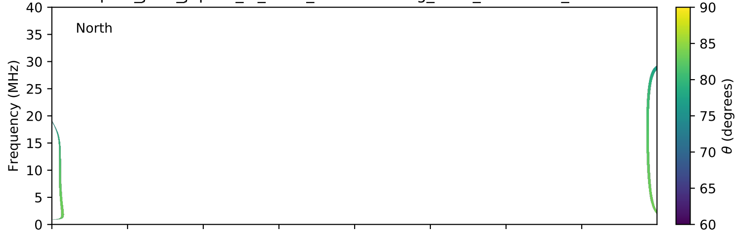
expres_juno_jupiter_io_isaac_lossc-wid1deg_3kev_20161209_v01.cdf
