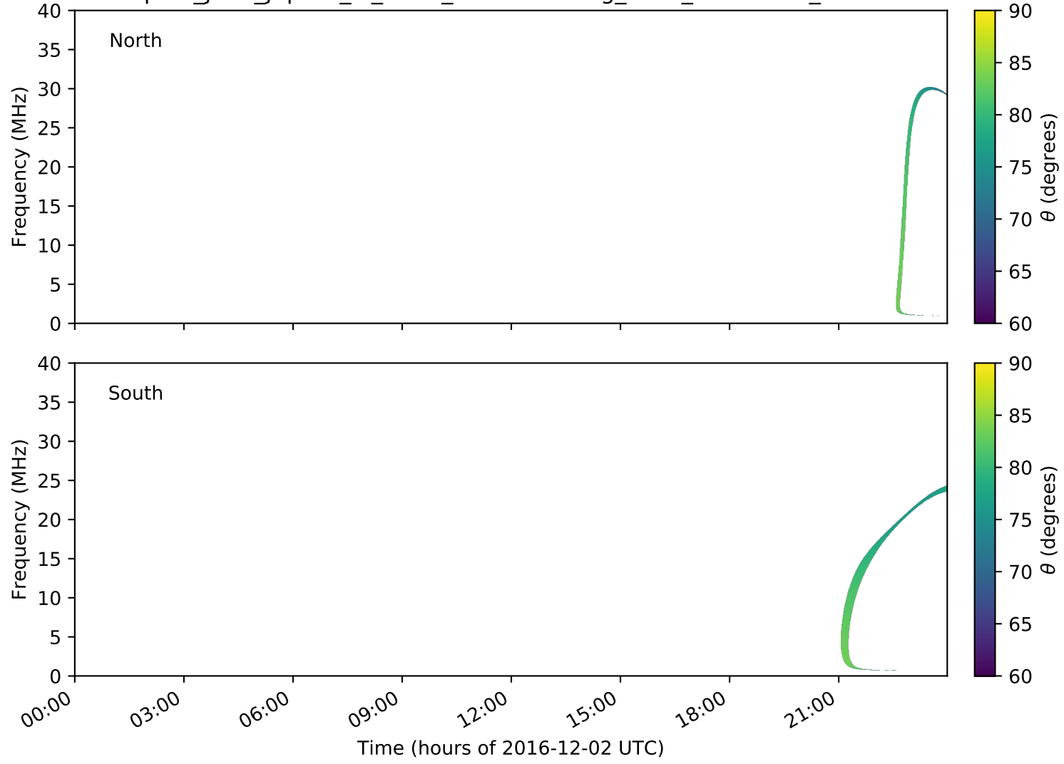
expres_juno_jupiter_io_isaac_lossc-wid1deg_3kev_20161202_v01.cdf
