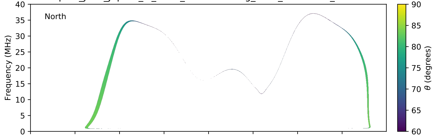
expres_juno_jupiter_io_isaac_lossc-wid1deg_3kev_20161201_v01.cdf
