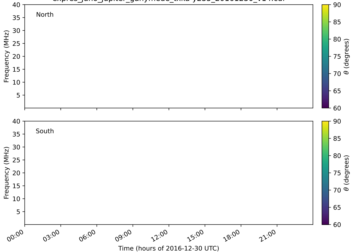
expres_juno_jupiter_ganymede_txka-y235_20161230_v14.cdf
