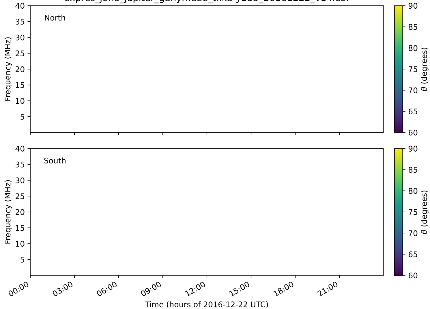
expres_juno_jupiter_ganymede_txka-y235_20161222_v14.cdf
