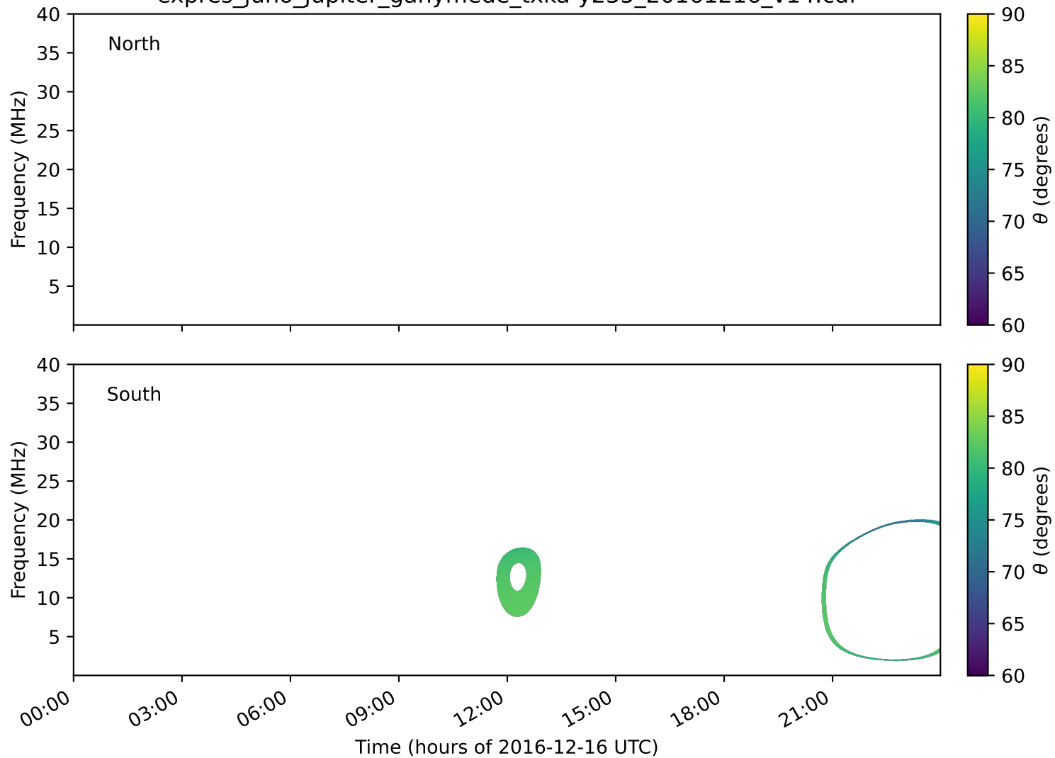
expres_juno_jupiter_ganymede_txka-y235_20161216_v14.cdf
