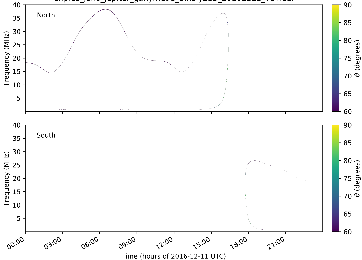
expres_juno_jupiter_ganymede_txka-y235_20161211_v14.cdf
