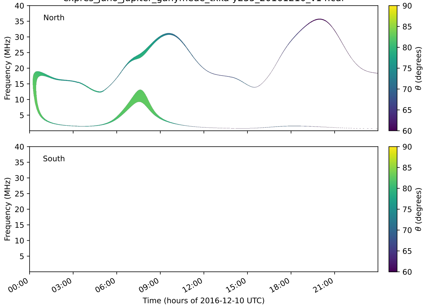
expres_juno_jupiter_ganymede_txka-y235_20161210_v14.cdf
