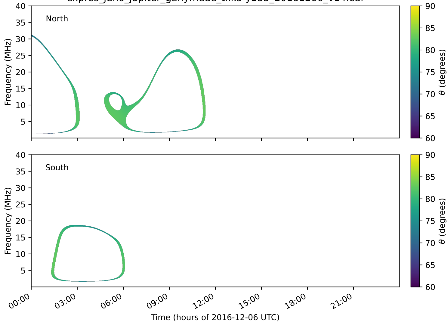
expres_juno_jupiter_ganymede_txka-y235_20161206_v14.cdf
