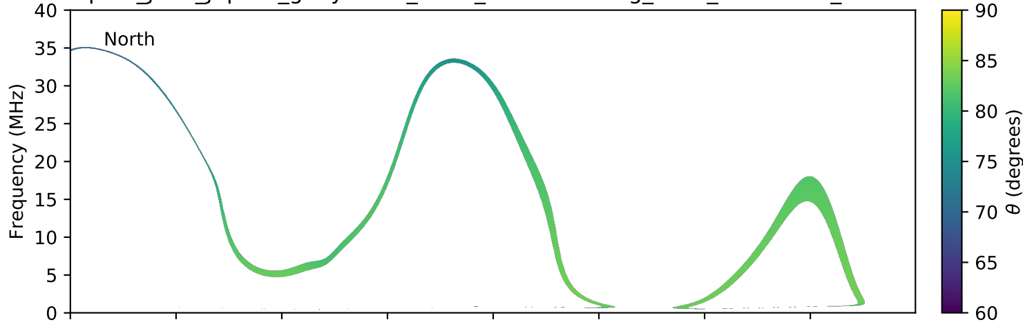
expres_juno_jupiter_ganymede_isaac_lossc-wid1deg_3kev_20161227_v01.cdf
