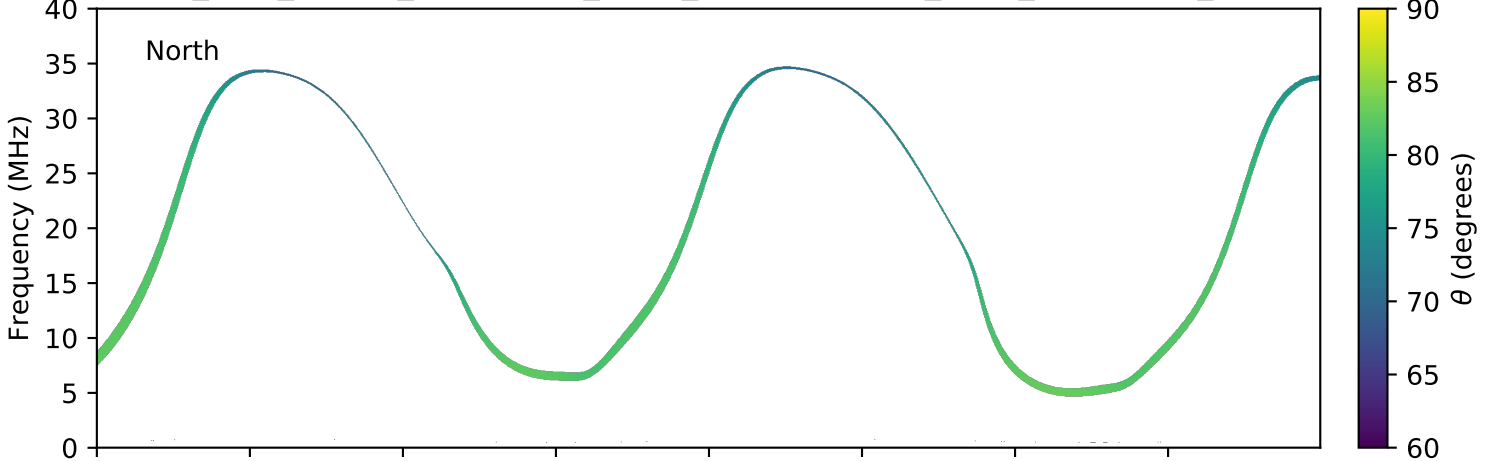
expres_juno_jupiter_ganymede_isaac_lossc-wid1deg_3kev_20161219_v01.cdf
