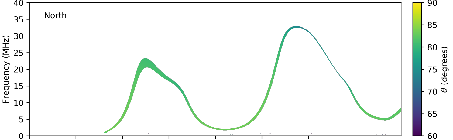
expres_juno_jupiter_ganymede_isaac_lossc-wid1deg_3kev_20161218_v01.cdf
