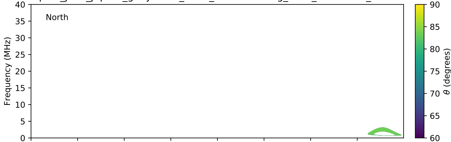
expres_juno_jupiter_ganymede_isaac_lossc-wid1deg_3kev_20161217_v01.cdf
