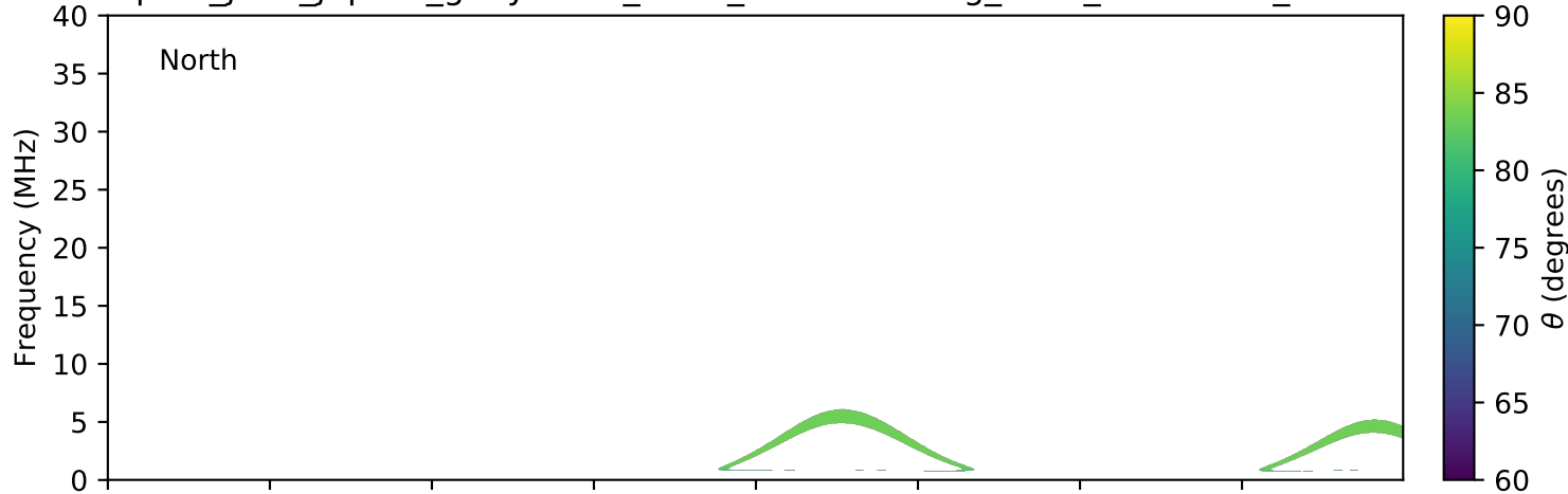
expres_juno_jupiter_ganymede_isaac_lossc-wid1deg_3kev_20161212_v01.cdf
