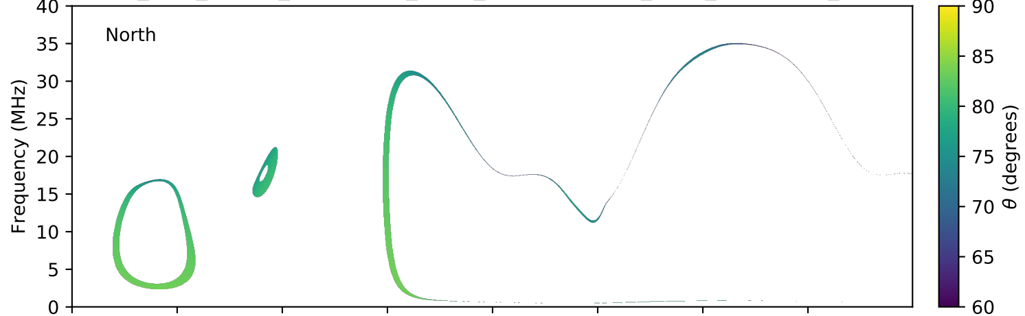
expres_juno_jupiter_ganymede_isaac_lossc-wid1deg_3kev_20161210_v01.cdf
