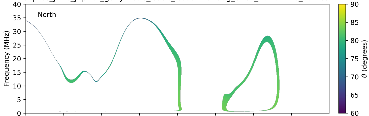
expres_juno_jupiter_ganymede_isaac_lossc-wid1deg_3kev_20161206_v01.cdf
