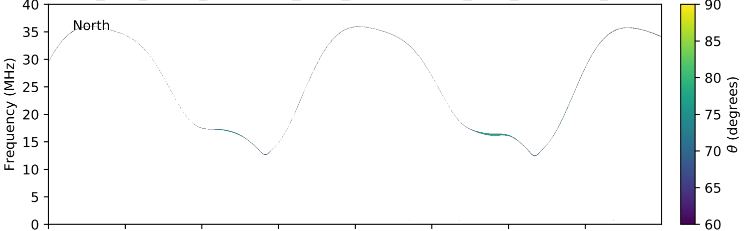
expres_juno_jupiter_ganymede_isaac_lossc-wid1deg_3kev_20161205_v01.cdf
