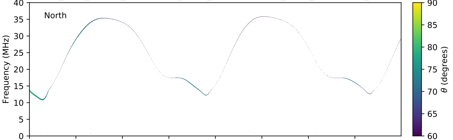
expres_juno_jupiter_ganymede_isaac_lossc-wid1deg_3kev_20161204_v01.cdf
