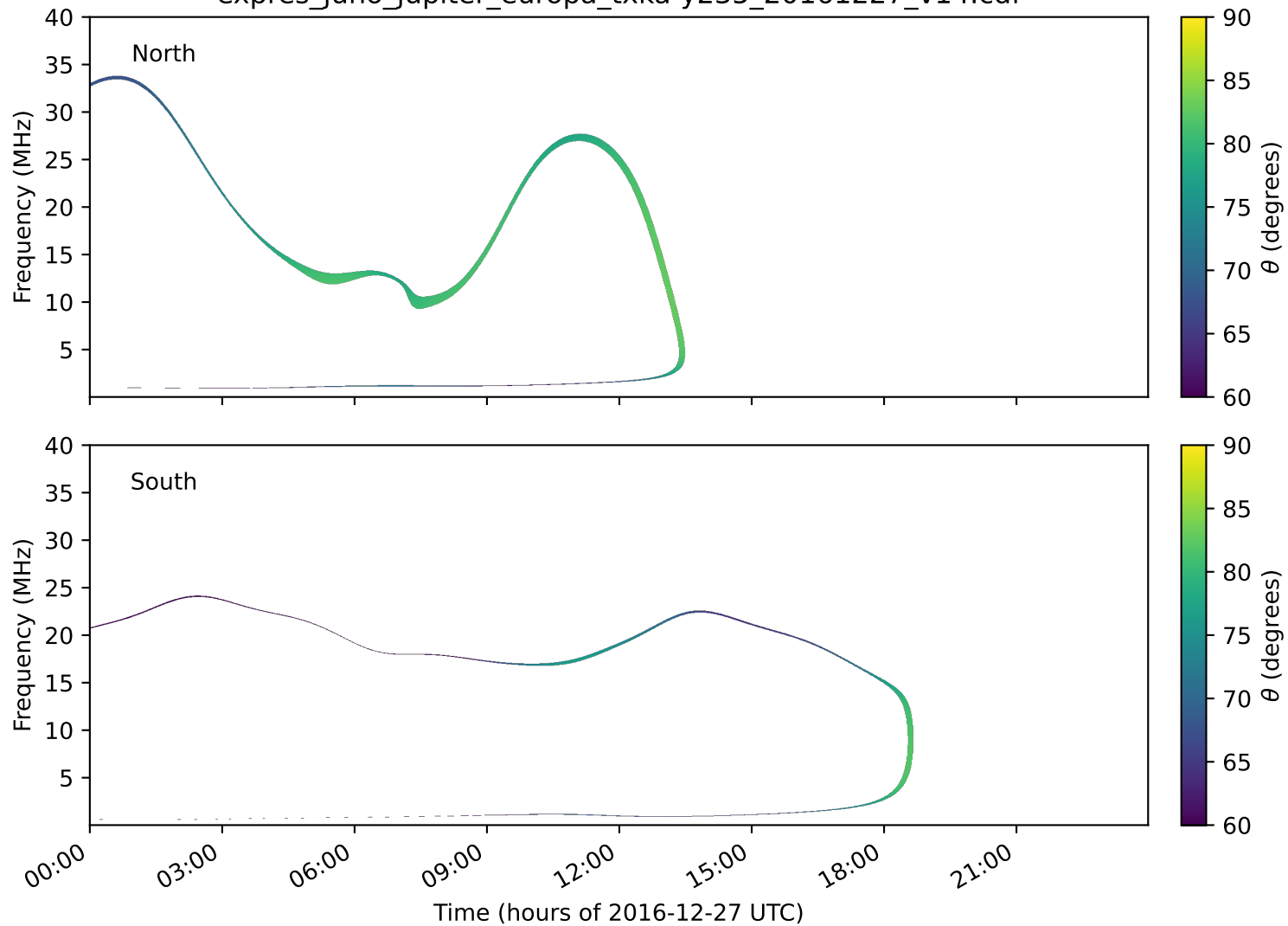
expres_juno_jupiter_europa_txka-y235_20161227_v14.cdf
