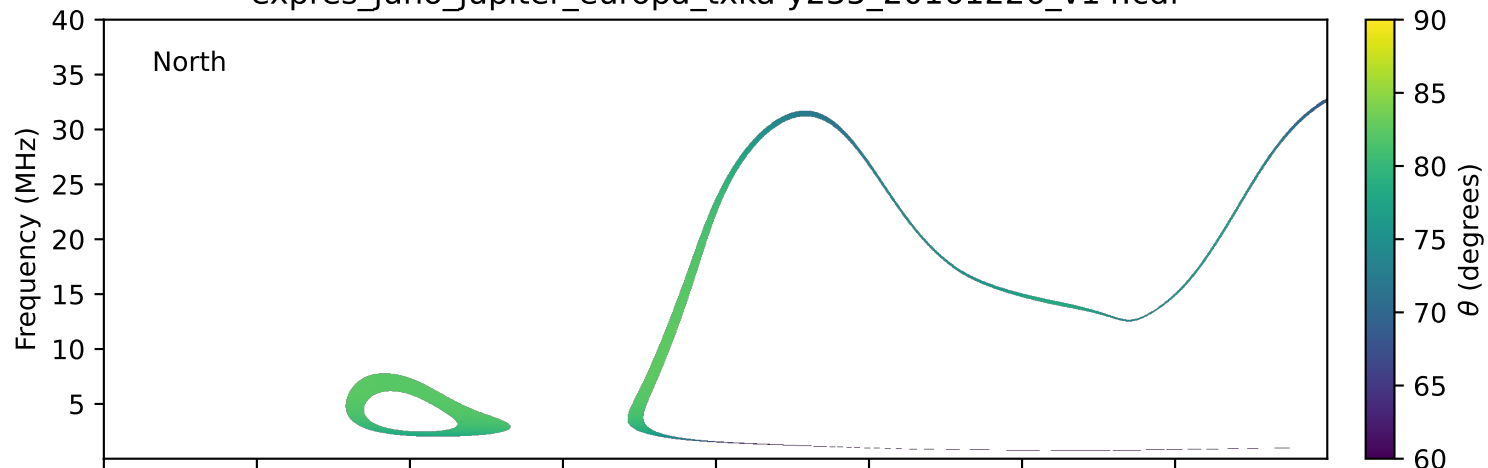
expres_juno_jupiter_europa_txka-y235_20161226_v14.cdf
