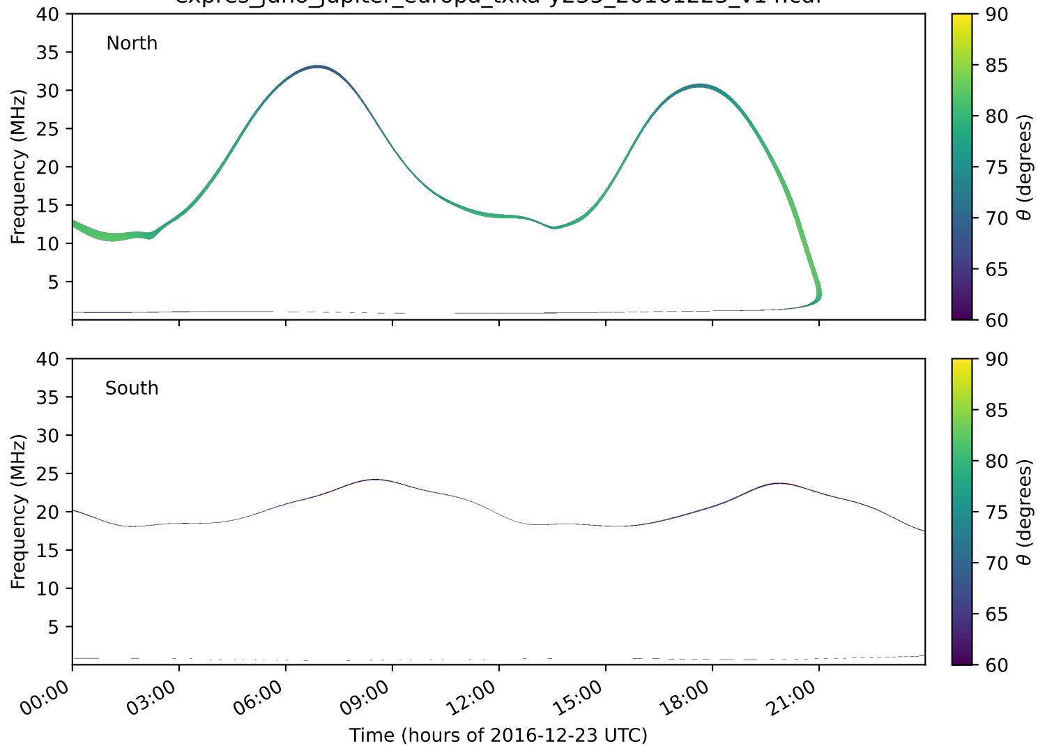
expres_juno_jupiter_europa_txka-y235_20161223_v14.cdf
