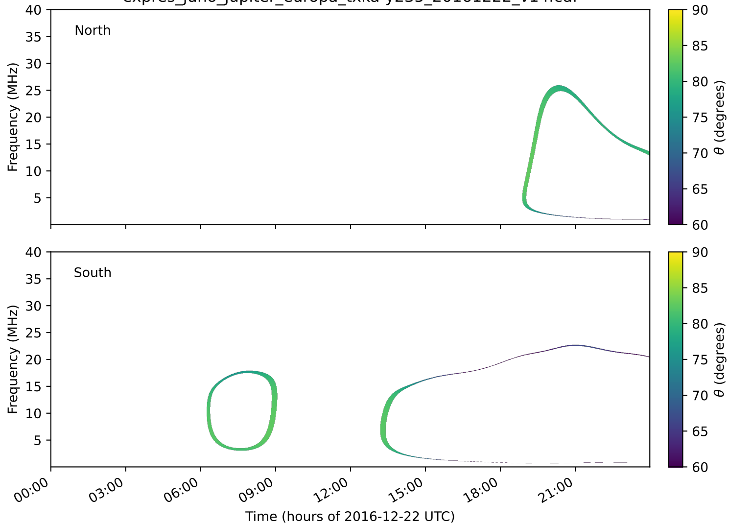
expres_juno_jupiter_europa_txka-y235_20161222_v14.cdf
