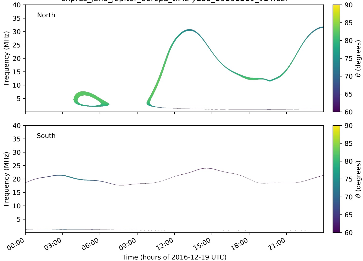
expres_juno_jupiter_europa_txka-y235_20161219_v14.cdf
