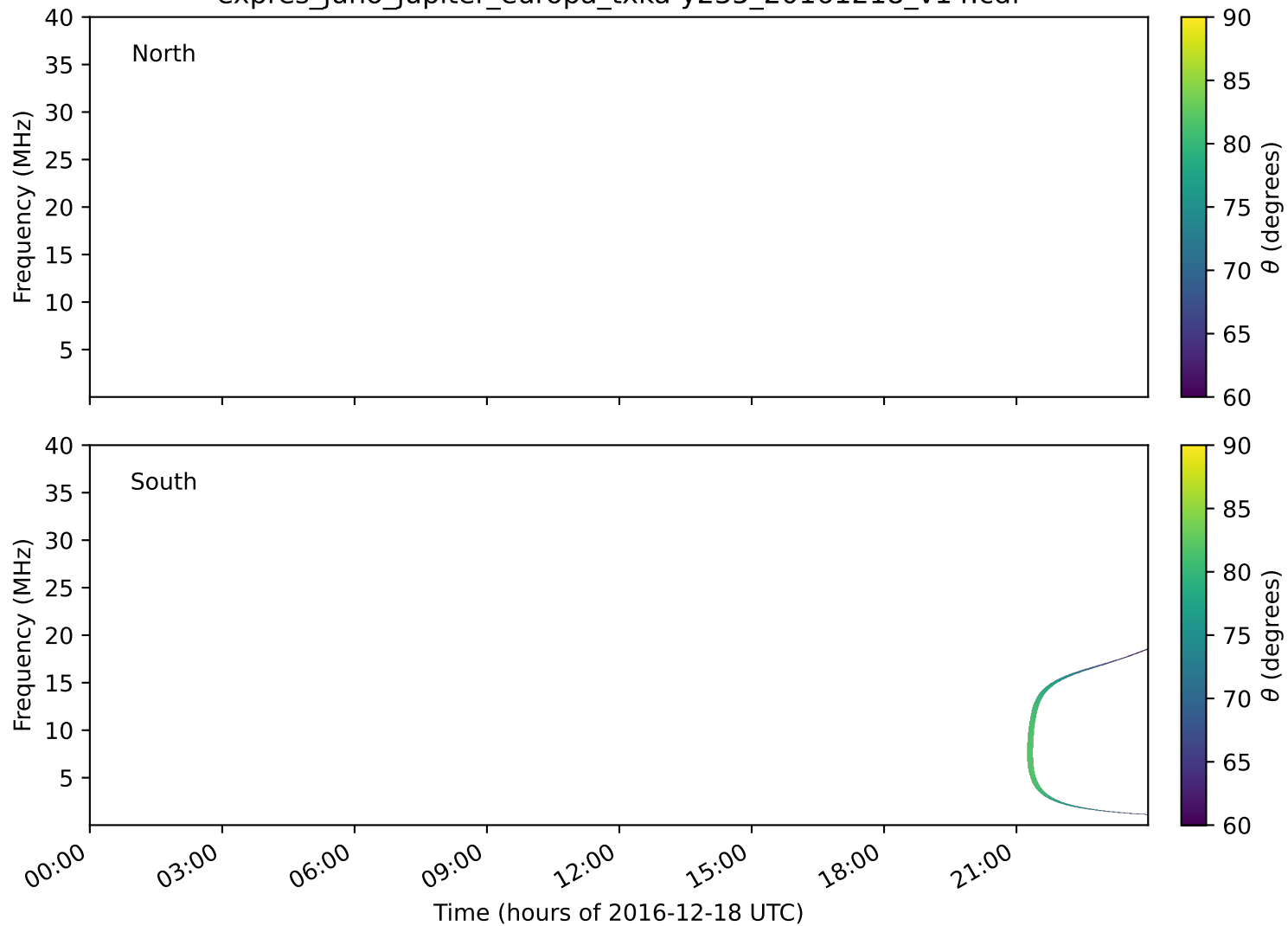
expres_juno_jupiter_europa_txka-y235_20161218_v14.cdf
