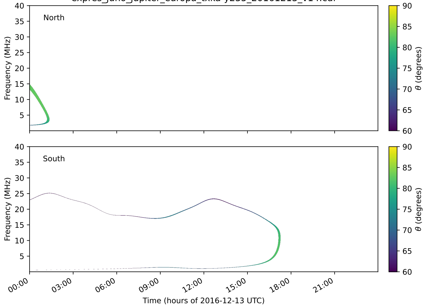
expres_juno_jupiter_europa_txka-y235_20161213_v14.cdf
