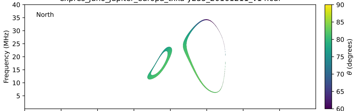
expres_juno_jupiter_europa_txka-y235_20161211_v14.cdf
